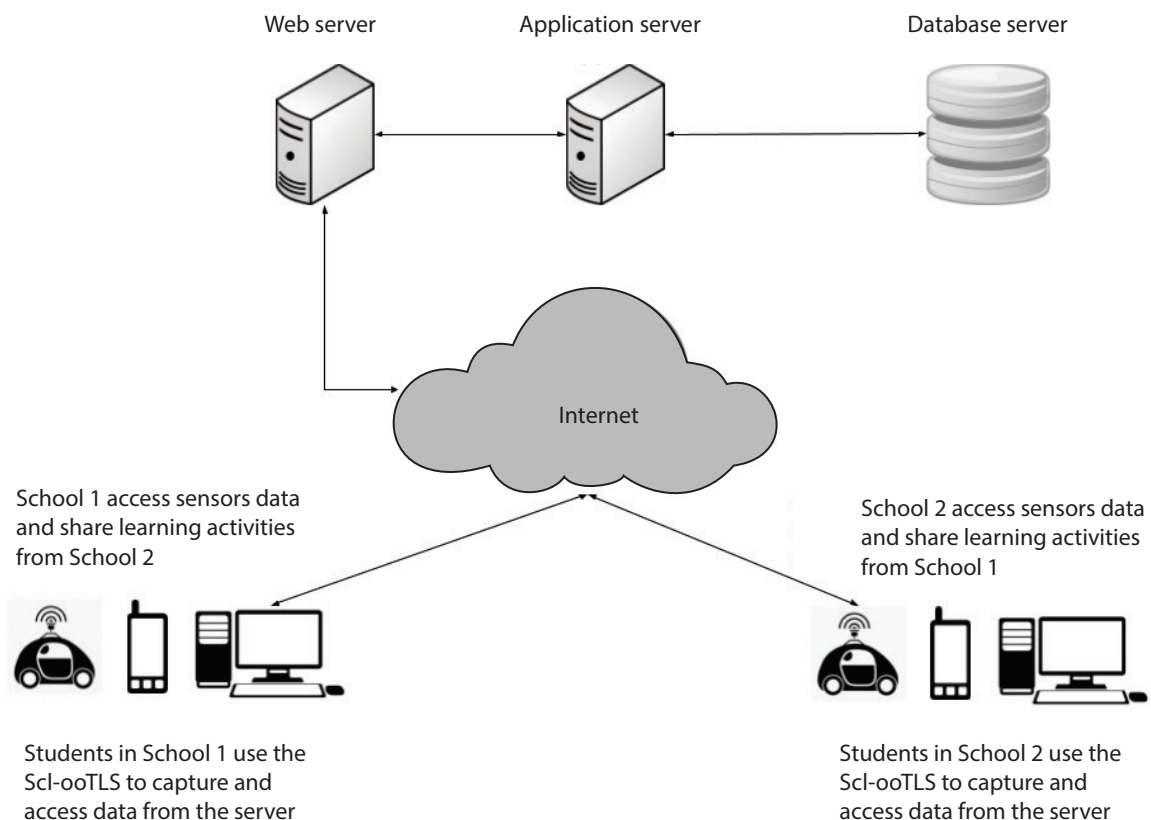
Figure 2 Quickscience System Architecture
