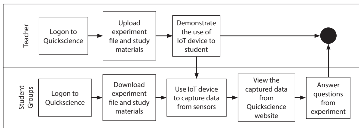
Figure 3 Quicksience activity diagram
