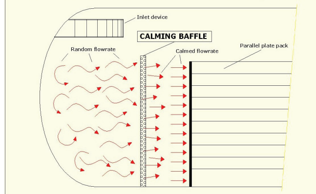
Figure 4 Effect of a calming baffle on a 2 phase liquid flow
