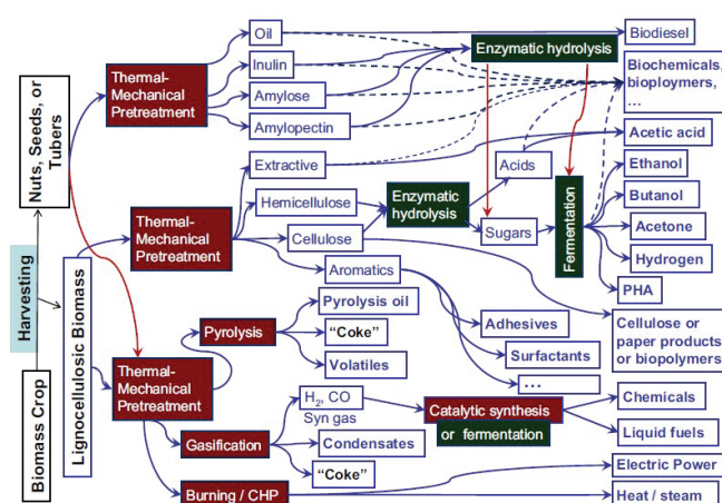
Fig. 1. A schematic description of biorefinery processes [5].
