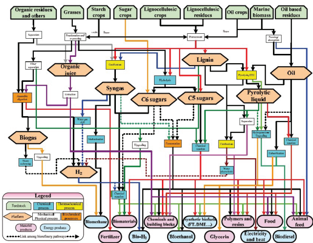
Fig. 2. Overview of the biorefinery classification system
