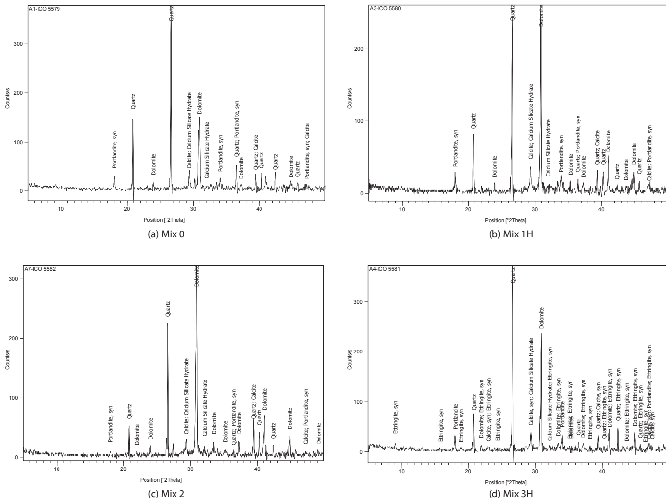
Figure 7 XRD of rubberised concrete specimens
