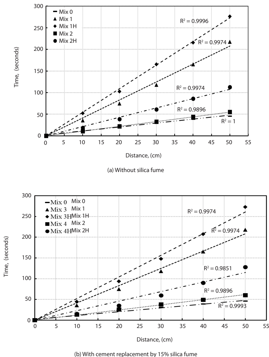
Figure 6 Indirect UPV for homogeneity testing
