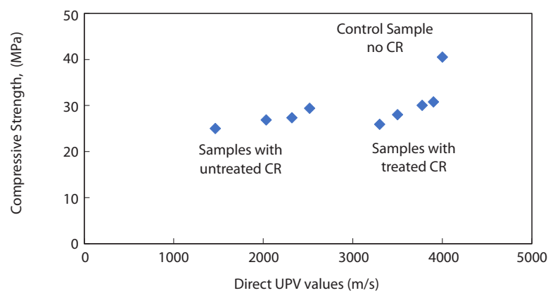
(b) Scatter diagram for the compressive strength and UPV values
